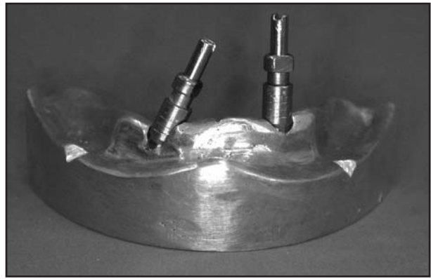
Fig. 1: Metallic matrix with two implants positioned at 65° and 90° in relation to the alveolar edge surface with square impression copings.
