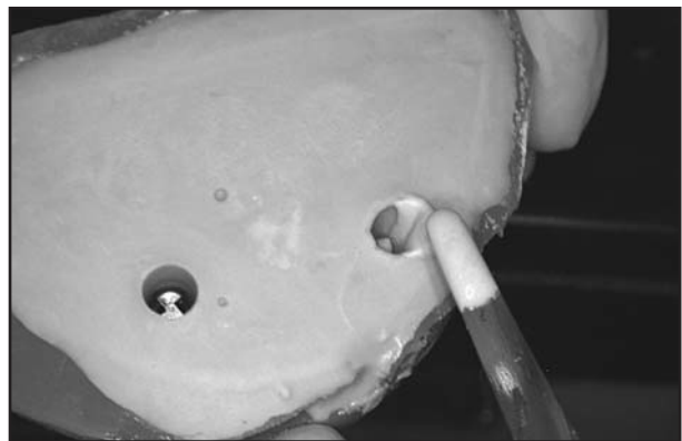
Fig. 3: Final dental stone pouring into the space created by the latex tube - group EP.
