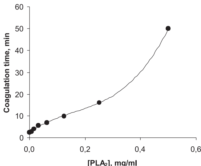
FIGURE 4. Delay in the clotting time of mice plasma previously incubated with purified enzyme from B. jararacussu venom. The clotting time of plasma by 0.25 M CaCl 2 corresponded to 2.5 minutes. Data show mean ± SD (n= 3) *P < 0.01 versus control plasma.
