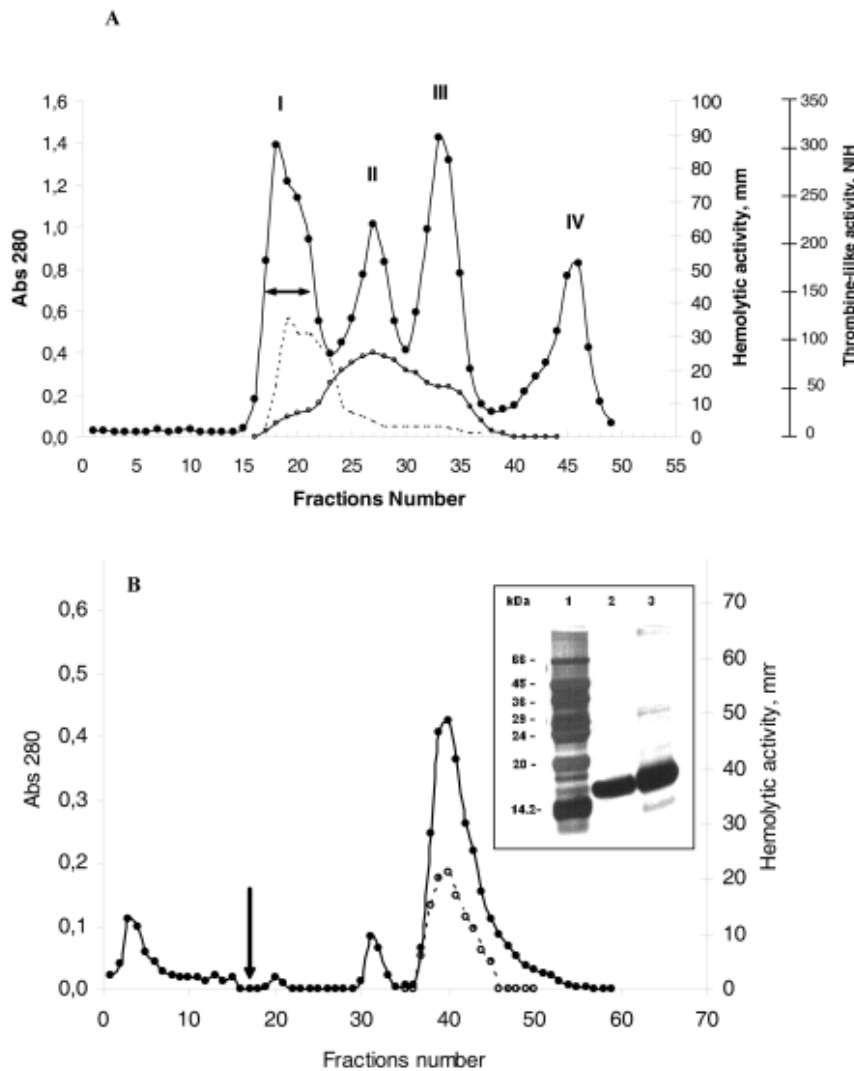
FIGURE 1. Isolation of phospholipase A 2 from B. jararacussu venom. (A) Twenty milligram of the venom dissolved in 250 \mu l of 10 mM sodium phosphate buffer, pH 7.2 was applied to a 1.0 x 50 cm column of Sephadex G-75 equilibrated with the buffer. The column was eluted with the same buffer and 0.75 ml fractions were collected. ●, Protein (Abs 280 nm); ⊖, hemolytic activity (diameter of the halo, mm); ---, thrombin-like activity (NIH). Double arrow indicates fractions that showed hemorrhagic activity. (B) Ion exchange chromatography of the pooled fraction (SIII) on column SP Sephadex C-25 previously equilibrated with 50 mM Tris, 100 mM KCl, pH 7.0. The column was eluted with a linear gradient of KCl from 0.1 to 0.5 M in the same buffer, pH 7. Arrow indicates change in elution buffer ●, Protein (Abs 280 nm); ⊖, hemolytic activity (diameter of the halo, mm). Insert SDS-PAGE at 15% (w/v), after reducing conditions. Molecular Mass Estimation. Lane 1, molecular mass markers: bovine serum albumin (66 kDa), egg albumin (45 kDa), glyceraldehydes-3-phosphate dehydrogenase (36 kDa), carbonic anhydrase (29 kDa), trypsinogen (24 kDa), trypsin inhibitor (20 kDa), and \alpha -lactalbumin (14,20 kDa). Lane 2, purified phospholipase A 2 obtained from the major peak of SP chromatography; Lane 3, fractions pool SIII. The gel was silver stained by the procedure of Blum et al. (1987).
