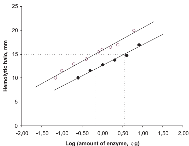
FIGURE 2. Effect of dose of B. jararacussu venom (○) and PLA 2 enzyme (●) on the indirect hemolytic activity in vitro . The DHM obtained from venom (0.66 mg) and from enzyme (3.66 mg) corresponding to the amount of venom or enzyme that induced a hemolytic halo of 15-mm diameter. Values are means of three determinations.
